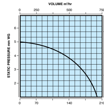
Performance Graph XFS230 Series 668m 3 /hr, 185 litres per second
