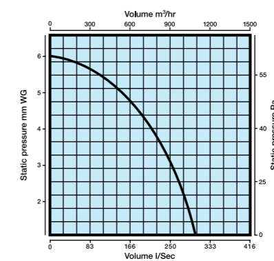
Performance Graph XFS300 Series 1100m 3 /hr, 306 litres per second
